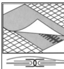
Flap-Over Seam
